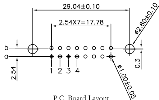
P.C. Board Layout (Tolerance: \pm 0.05 )
