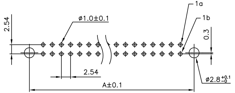
RECOMMENDED P.C.B LAYOUT(TOP VIEW) TOLERANCES: ±0.10mm
