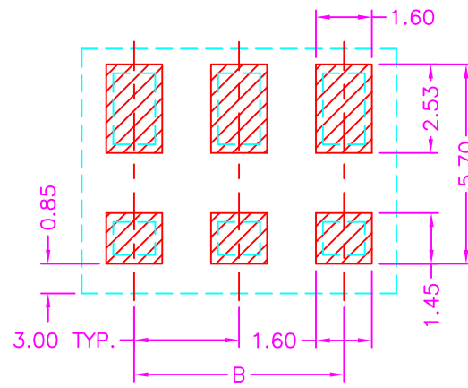
P.C.B. LAYOUT TOP VIEW \pm 0.05
