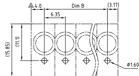
PCB LAYOUT
