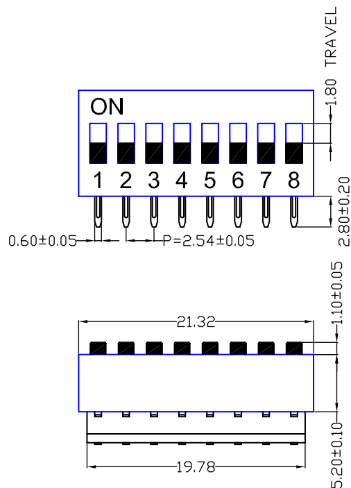
WIRING DIAGRAM
