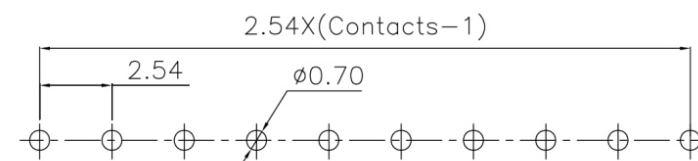
PCB Layout
