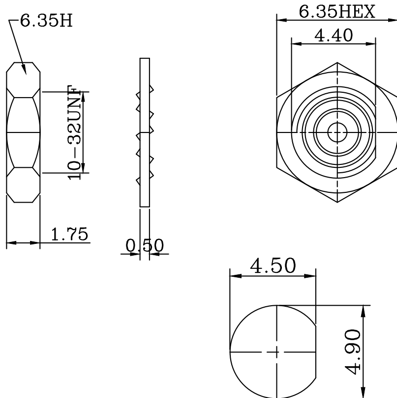
MOUNTING HOLE
