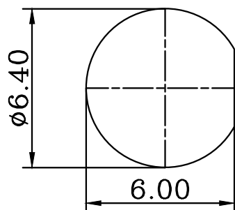
MOUNTING HOLE
