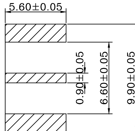
RECOMMENDED FOOTPRINT
