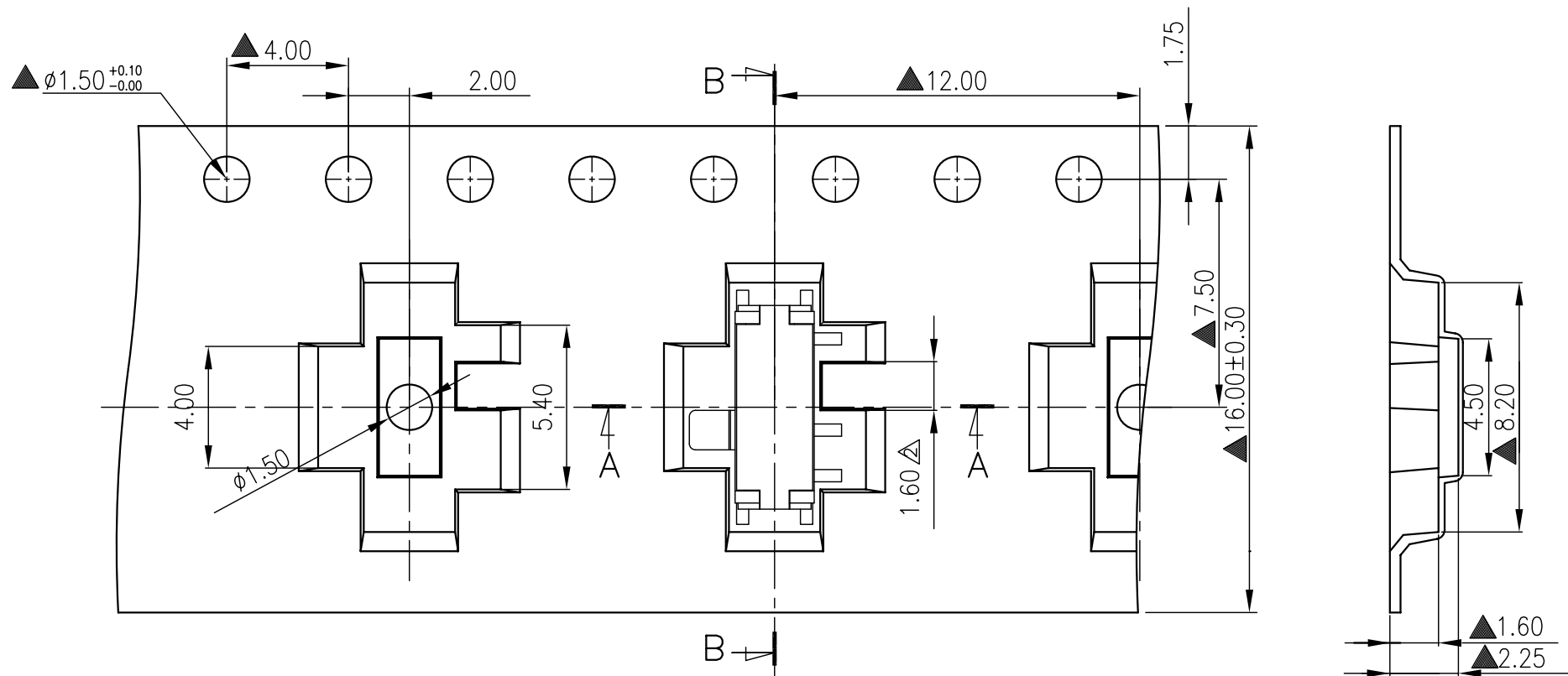
B-B Section
