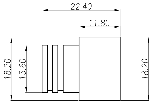
HOUSING
