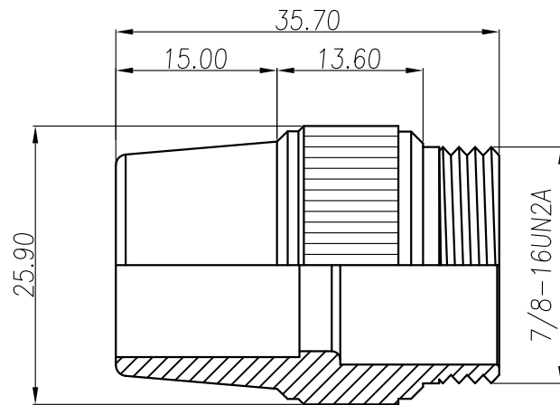
SHELL
