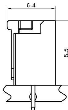
Mated Height(REF.)
