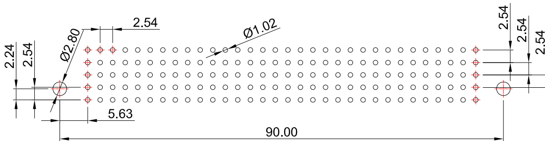
PCB LAYOUT
