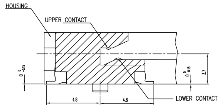
SECT "A"- "A" (S=4/1)
