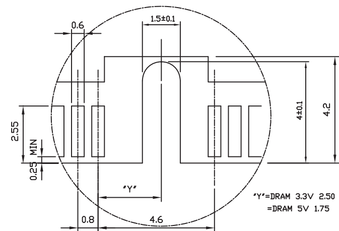
DETAIL X
