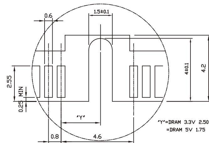
DETAIL X
