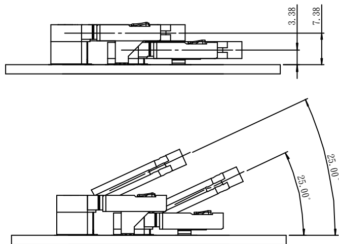
DDR S.O. DIMM 200P 5.2&amp;9.2 OVERLAY FIGURE
