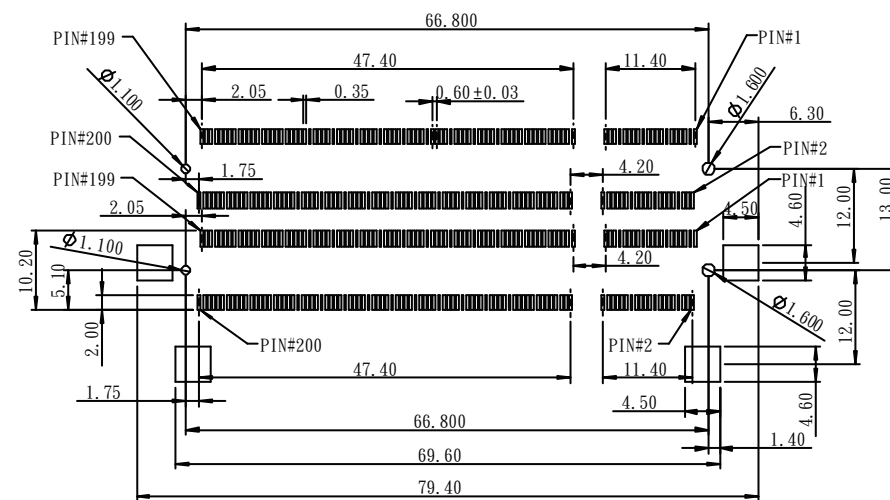
PCB LAYOUT : COMPONENT SIDE(4.0&amp;8.0 TYPE)
