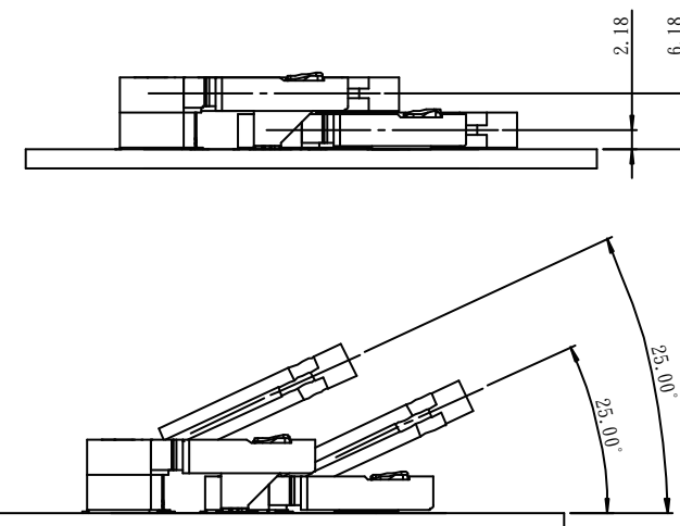
DDR S.O. DIMM 200P 4.0&amp;8.0 OVERLAY FIGURE
