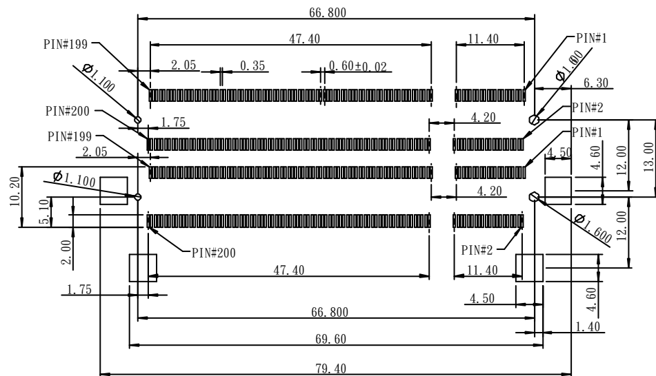
PCB LAYOUT : COMPONENT SIDE(5.2&amp;9.2TYPE)
