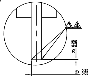
DETAIL "C" SCALE 5:1
