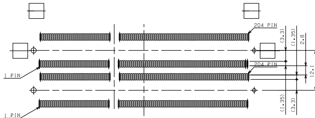
推奨基板レイアウト寸法 RECOMMENDED MOUNTING P.C. BOARD PATTERN LAYOUT DIM.
