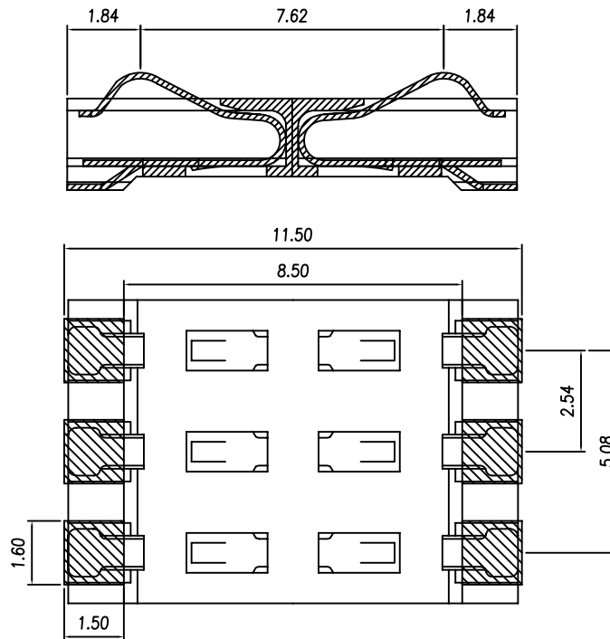
PCB PAD LAYOUT
