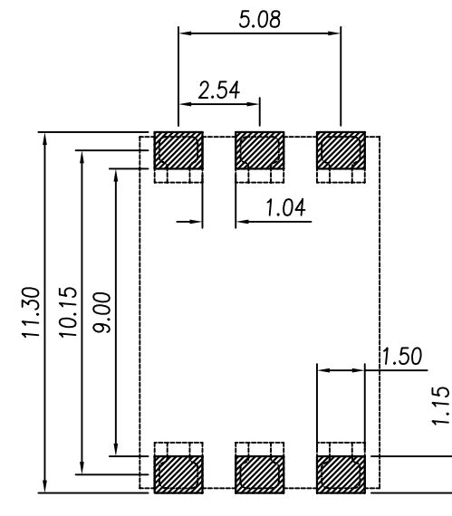
PCB PAD LAYOUT
