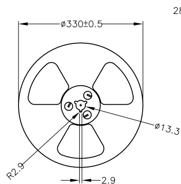
REEL FOR CARRIER TAPE
