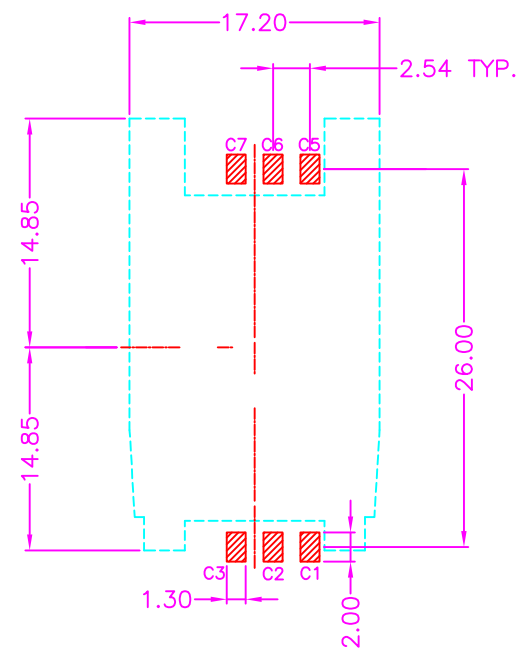
P.C.B. LAYOUT TOP VIEW ±0.05
