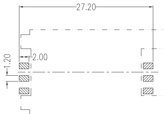
RECOMMEND P.C.B. LAYOUT TOP VIEW
