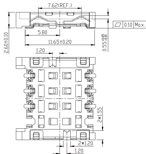
Figure 5.1 Mechanical outline dimension (6 pins)
