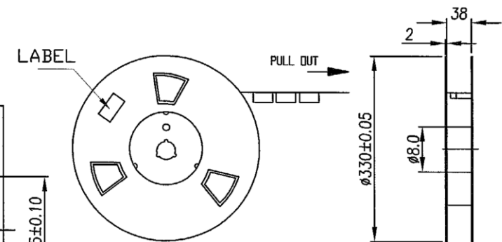
Reel Form Diagram
