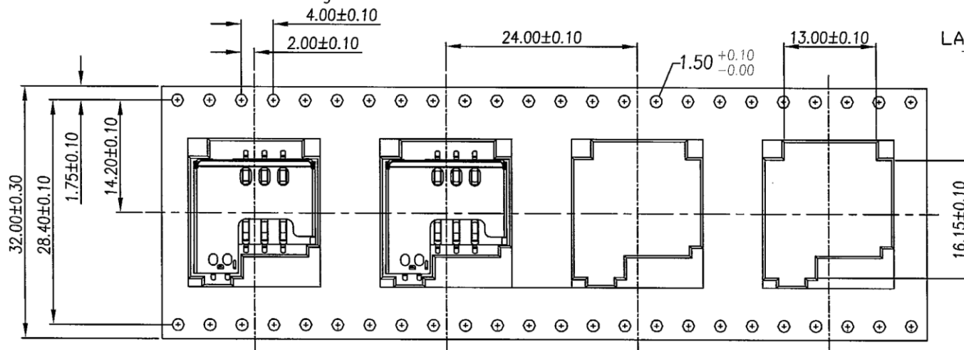
Embossed Tape Carrier Diagram Carrier Dimensions Diagram
