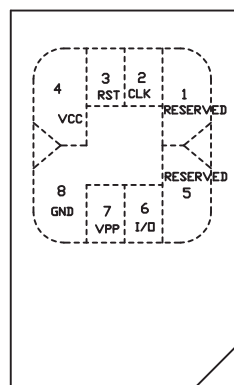
SIM CARD 2:1 TOP VIEW
