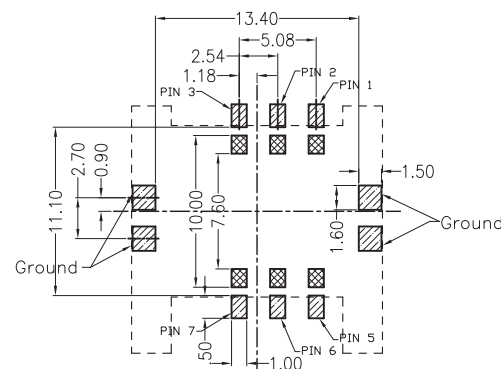
RECOMMENDED P.C.B HOLE LAYOUT COMPONENT SIDE VIEW(TOLERANCE: +/-0.05)
