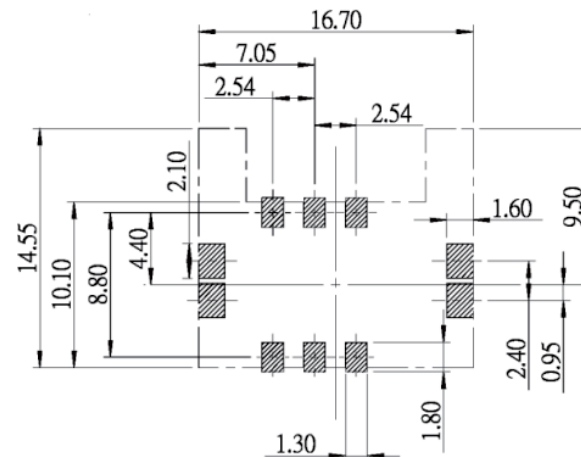
PCB PATTERN LAYOUT GENERAL TOLERANCE : \pm 0.05
