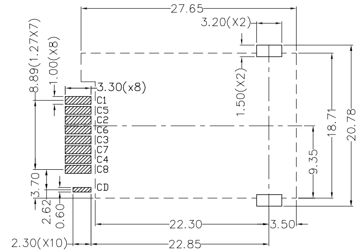
RECOMMENDED P.C.B LAYOUT COMPONENT SIDE(TOLERANCE ±0.05)
