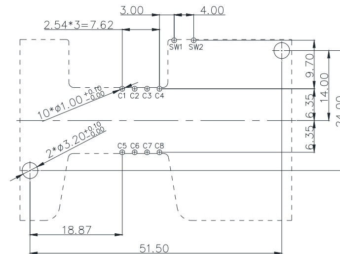
Unit: mm; Tolerances: \pm 0.05 mm Figure 5.2 Reference dimension for PCB layout
