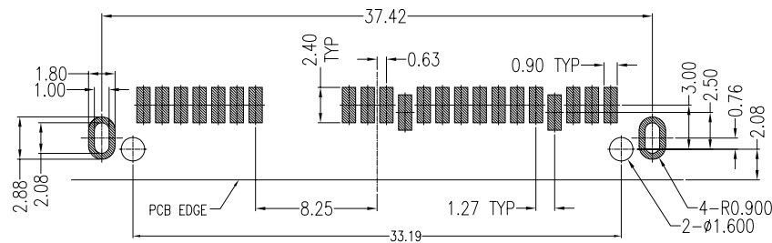
P.C.B. LAYOUT (T=1.2)
