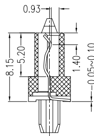
SECT B-B
