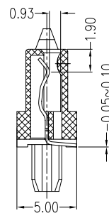
SECT C-C
