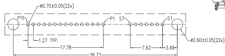
PCB LAYOUT COMPONENT SIDE
