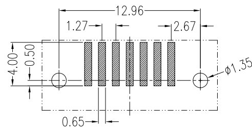
PCB LAYOUT (T=1.60mm)
