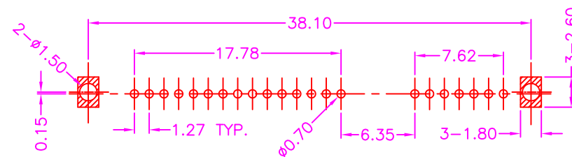
P.C.B. LAYOUT TOP VIEW ±0.05
