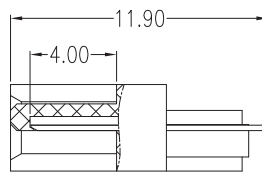
SECT C-C
