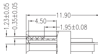
SECT B-B
