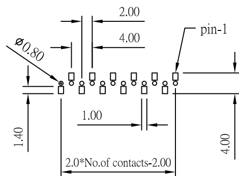
Recommended P.C. Board SMD Layout
