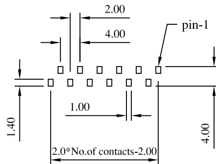
Recommended P.C. Board SMD Layout
