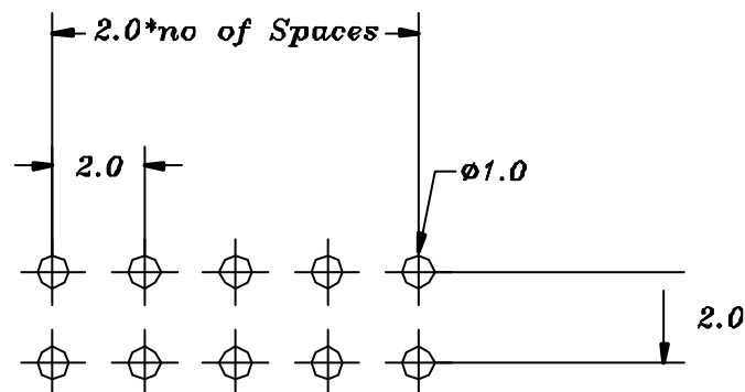
Pc Board Layout(Dual Row)
