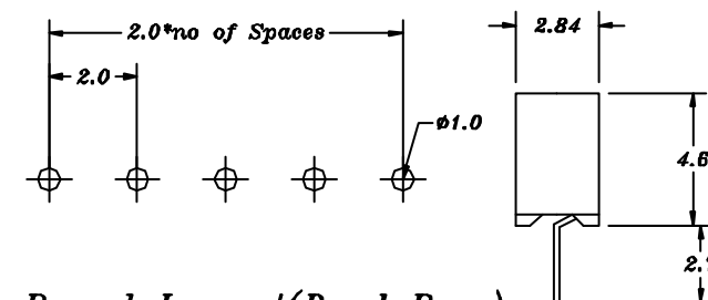
PC Board Layout(Dual Row)
