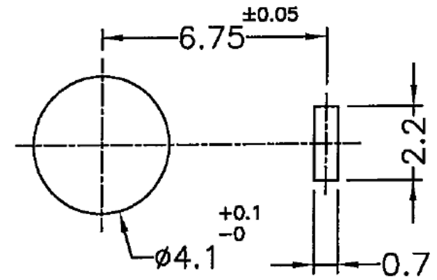
MOUNTING HOLE
