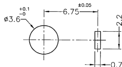
MOUNTING HOLE
