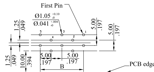
R Type PCB special layout for reverse
