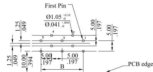
L Type PCB layout for reverse
