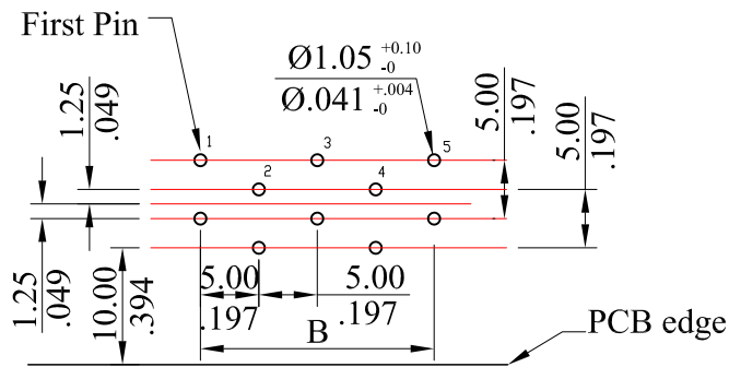
PCB layout for normal
