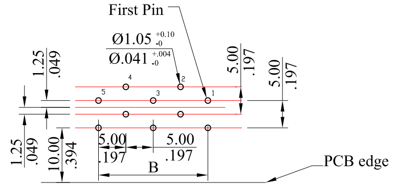
PCB layout for reverse
