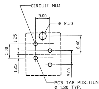
TYPE-1 P.C. BOARD LAYOUT (2P)
