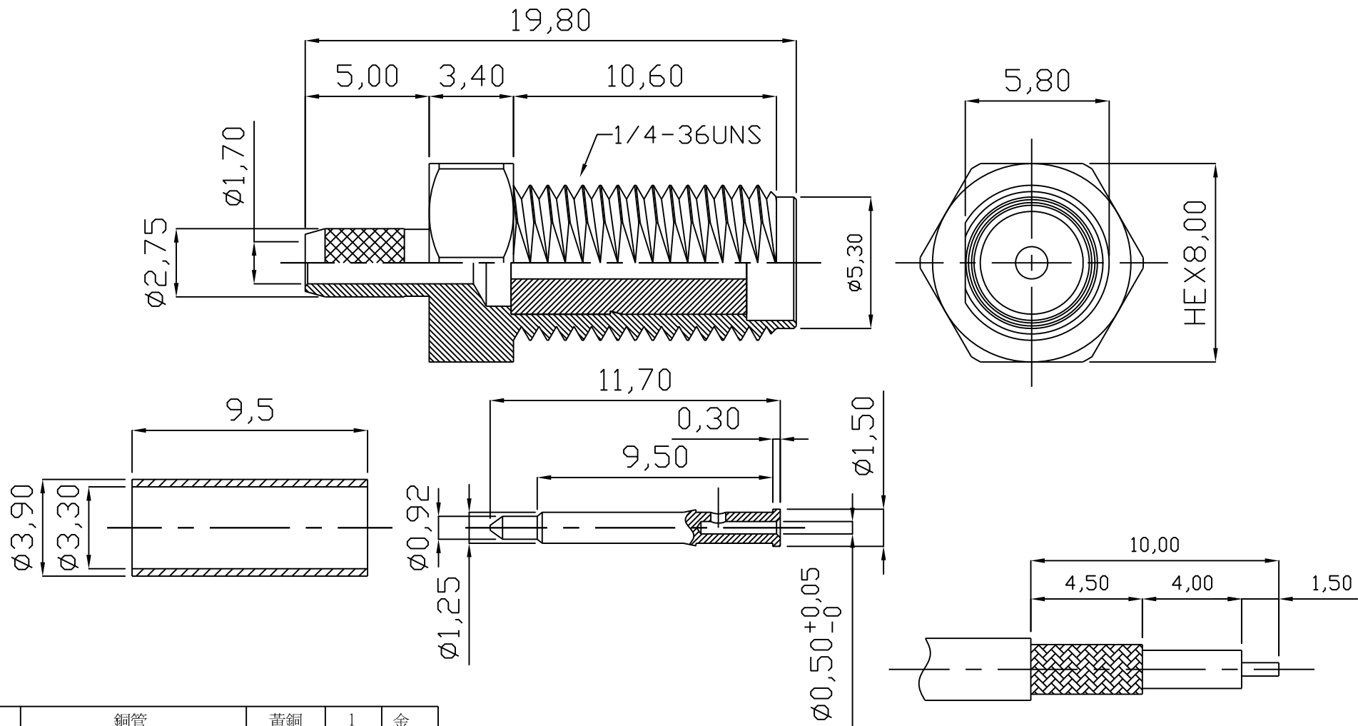
RG-316u / RG-174 Recommended Cable Strip
