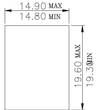
Single Panel-Latch Clearance Panel Thickness 0.062 inch
