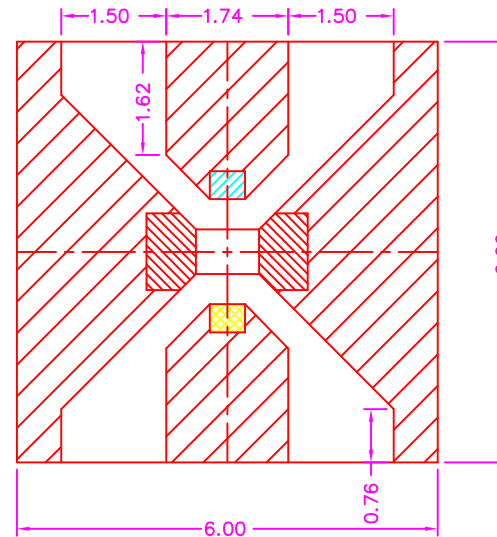
P.C.B. LAYOUT TOP VIEW \pm 0.05
