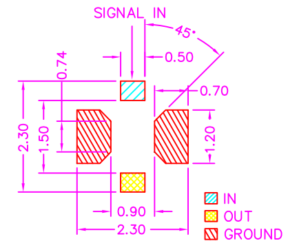
RECOMMEND STENCIL MASK PATTERN (MASK THICKNESS 0.10~0.12mm)
