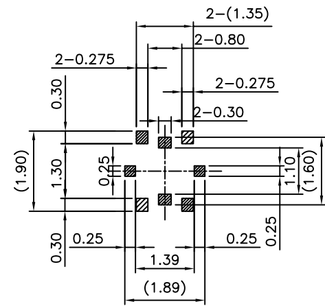
Recommnd Stencil Mask Pattern (Mask Thickness 0.10mm)
