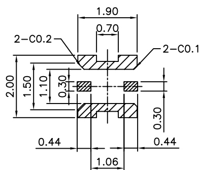
Recommnd PCB Layout
