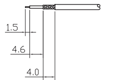
RECOMMENDED CABLE STRIPPING DIM
