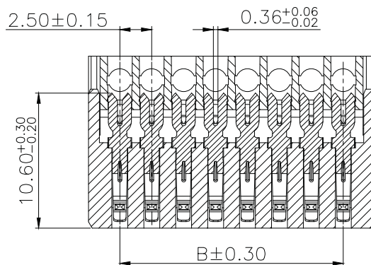
SECTION E-E
