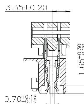
SECTION F-F
